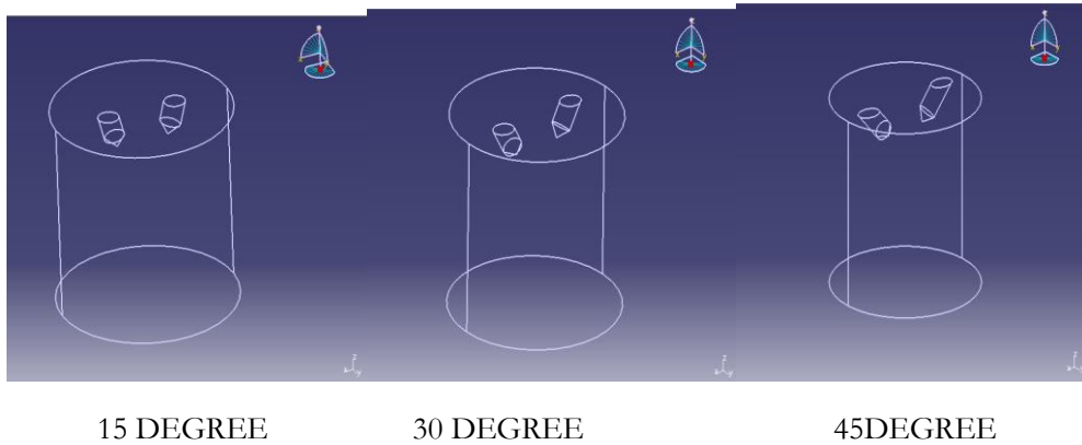
Fig 3D model Diesel Spray injectors in various angles
